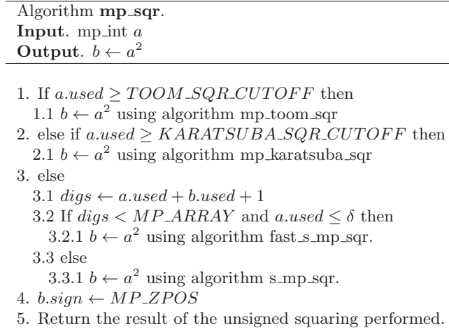
Figure 5.15: Algorithm mp_sqr
